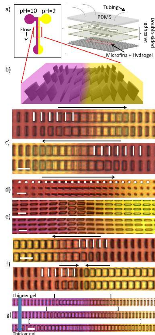
Fig. 2 Patterning and actuation of microstructures driven by a pH-responsive hydrogel induced by a pH gradient, which was created by flowing acid and base in a microfluidic channel. a) Schematic representation of experimental setup. b) 3-D schematic showing an orientation of microfins within such a microfluidic channel, as demonstrated in (c). c-g) Optical microscope images of actuated microstructures taken normal to the surface, showing that the direction of microstructure bending is always towards the acid. White lines or dots are place markers for the base of the structures to help visualize bending directions; bending directions are also marked with arrows above the micrographs. Color in all micrographs arises from pH indicator, bromophenol blue. Scale bars = 10 \mu\text{m} : c) Bending direction can be switched by pH interface reversal: microfins are bending to the right when the acid is flowed on the right side of the channel (top), and the same fins are bending to the left when the acid is flowed on the left side of the same channel (bottom). d) Microposts showing the same behavior as the microfins and bending toward lower pH. e) Microfins like those in (c) but placed at different angles relative to the laminar flow interface exhibiting different bending angles. f) When a sample, which actuates in response to homogeneous pH as shown in Figure 1b, is put in a pH gradient, it exhibits either a uniform bending direction corresponding to the bending direction of the original structures (e.g. to the left in the top image, when the acid is flowed to the left), or unique backward-bending at the base/acid interface, when the acid is flowed against the original bending direction, to the right. g) A surface in which there is gradient hydrogel thickness; as the gel thickness increases, the width of the region in which structures bend (indicated by brackets above the micrographs) also increases given the same pH interface.
