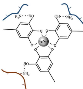
TA/Ag NPs
