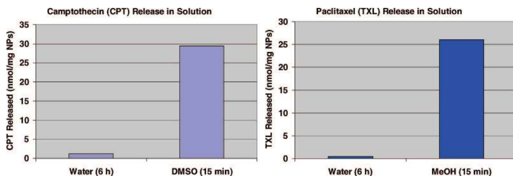
Figure 7. UV/vis absorption measurements show that most of the water-insoluble drug molecules were trapped inside the pores when the NPs were dispersed in water, but they were quickly released in organic solvents.
