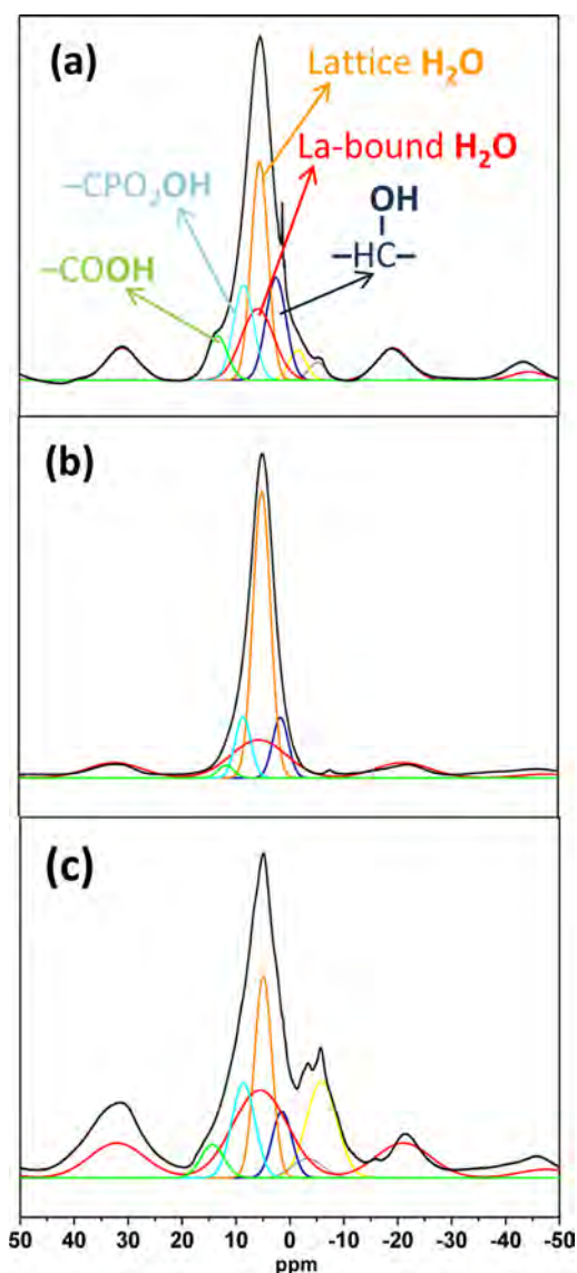
Figure 10. ^1\text{H} MAS NMR spectra, showing the fitting to several components for (a) LaHPA-II, (b) LaHPA-I at room temperature; (c) LaHPA-I heated at 80 °C. for 60 min. The bands situated close to -5 ppm are due to the signal probe and they are more conspicuous in panel c.
