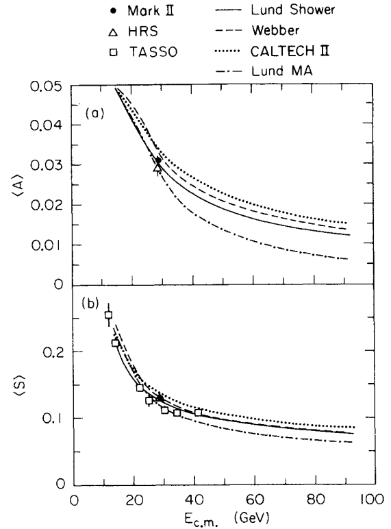
FIG. 27. (a) The \langle aplanarity \rangle and (b) \langle sphericity \rangle as a function of E_{c.m.} in comparison with HRS and TASSO results and the model predictions.
