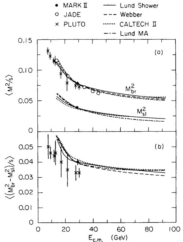
FIG. 28. (a) The \langle M_{br}^2/s \rangle and \langle M_{sl}^2/s \rangle , and (b) \langle (M_{br}^2 - M_{sl}^2)/s \rangle as a function of E_{c.m.} in comparison with PLUTO and JADE results and the model predictions.
