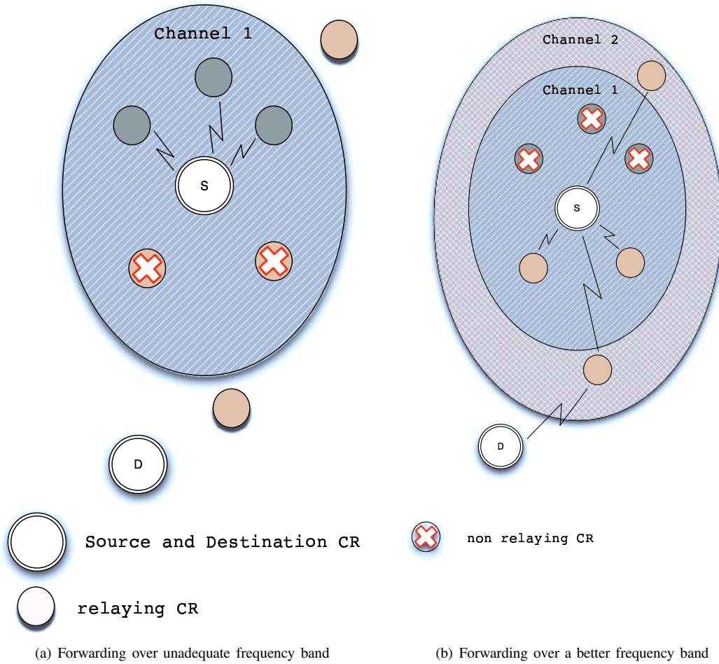
Fig. 5. Forwarding over two different channels in a multihop cognitive radio network. A different subset of receiver is obtained by selecting different radio bands.
