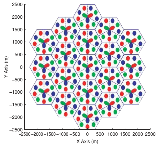
Figure 2 Frequency reuse pattern in non-transparent relay system.
