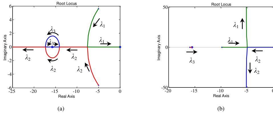
Fig. 7 Root locus diagrams for (a) k_{p\theta}, k_{pf}=1 \cdot 10^{-5}, k_Q=2.15 \cdot 10^{-4} and (b) k_{pf}, k_{p\theta}=2 \cdot 10^{-8}, k_Q=2.15 \cdot 10^{-4} .
