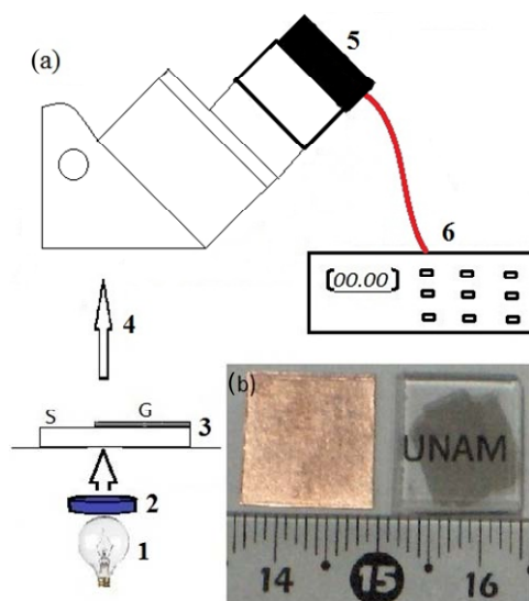
Figure 2. (a) Experimental arrangement for transmittance measurement: 1: light source; 2: filter; 3: sample where S means Substrate and G Graphene; 4: transmitted light collected by the objective of the microscope; 5: photodiode in place of the objective of the microscope; 6: electrometer. In (b), samples obtained by CVD on Cu and fused quartz (right) for optical characterization.
