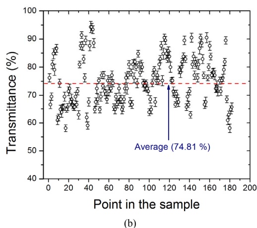
Figure 5. Homogeneity analysis, in (a) we show a digital image obtained by transmission of multilayer graphene films on top of a fused quartz substrate in (b) the value of the transmittance obtained from the digital image is shown.
