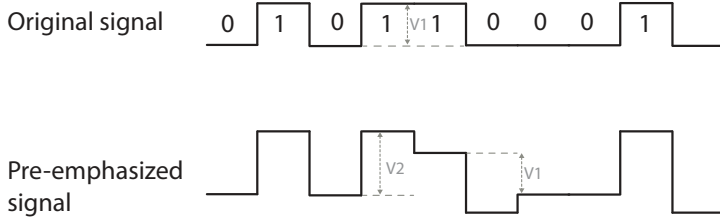
Figure 3.4: Explanatory diagram of pre-emphasis and de-emphasis using time-domain waveforms.
