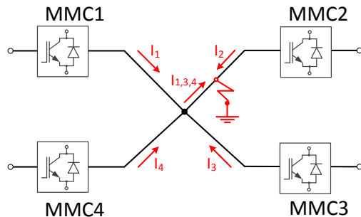
Fig. 10. Current direction during a dc fault [34].
