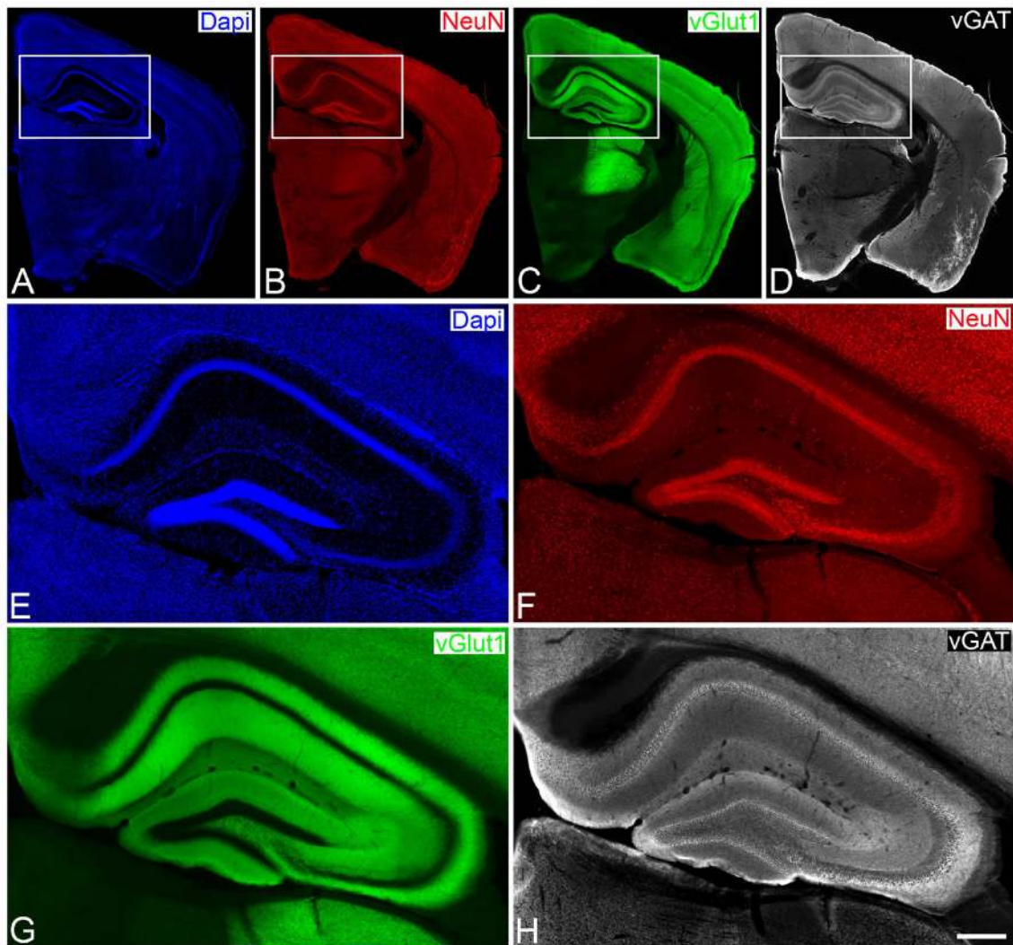
FIGURE 1 | Low- ( A–D ) and higher- ( E–H ) power photomicrographs obtained with a conventional fluorescence microscope (tile scan; 10x objective), showing patterns of Dapi staining, and NeuN and vGat immunostaining of a brain section from a vGlut1-transgenic mouse. The hippocampal region, squared zones in A–D , is shown at higher magnification in E–H , respectively. Scale bar (in H ): 1,200 \mu m in A,B ; 275 \mu m in E–H .
