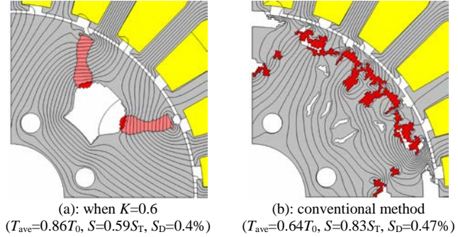
Fig. 12. Resultant rotor shapes obtained by different settings.
