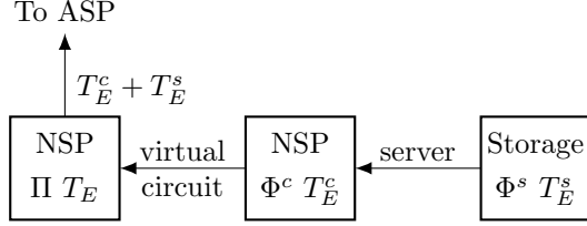
Figure 12: Propagation of control times to the ASP.
