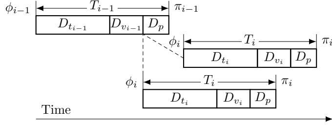
Figure 9: Schedule constraints.
