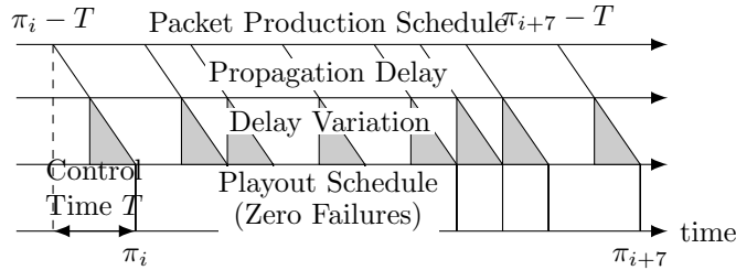
Figure 4: Illustration of incurred packet delays.
