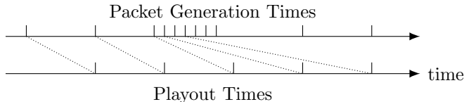
Figure 6: Limited channel capacity: Adjustment of retrieval times.
