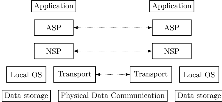
Figure 10: Relationships between synchronization components.
