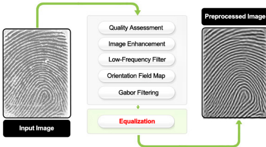
Figure 22: Flow diagram of the correlation-based pre-processing technique.
