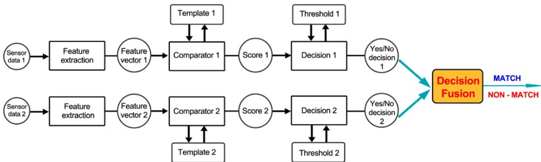
Figure 39: Fusion at decision level [7].
