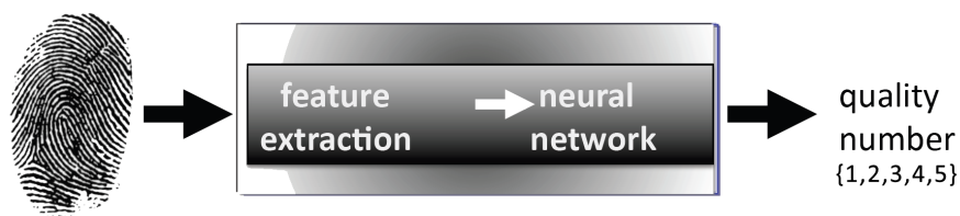
Figure 45: NIST Fingerprint Image Quality (NFIQ).
