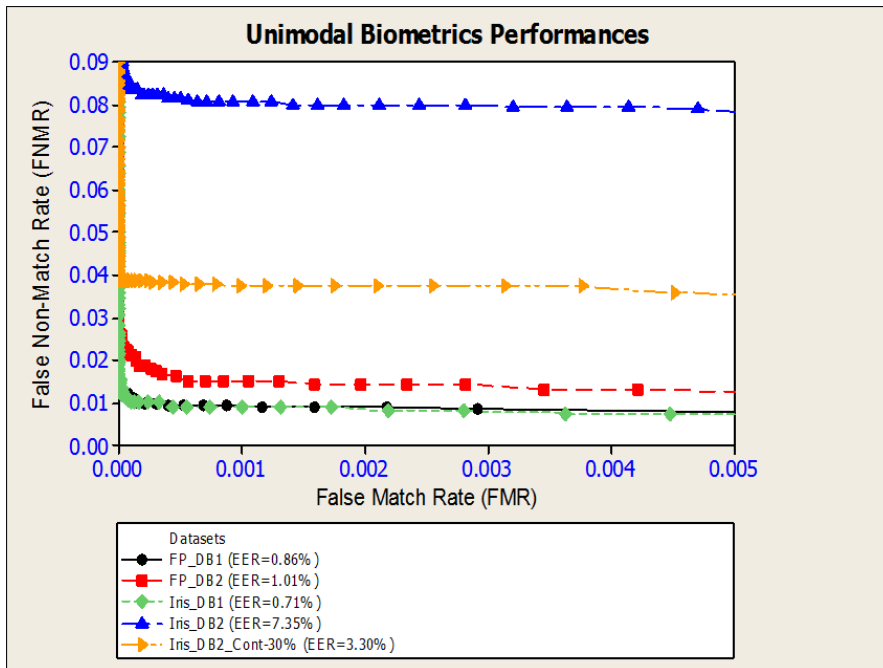
Figure 70: Comparison of Fingerprint and Iris Databases.
