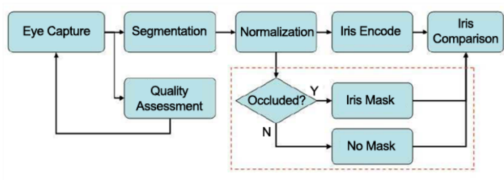
Figure 26: The block diagram of a generic iris recognition system [6].
