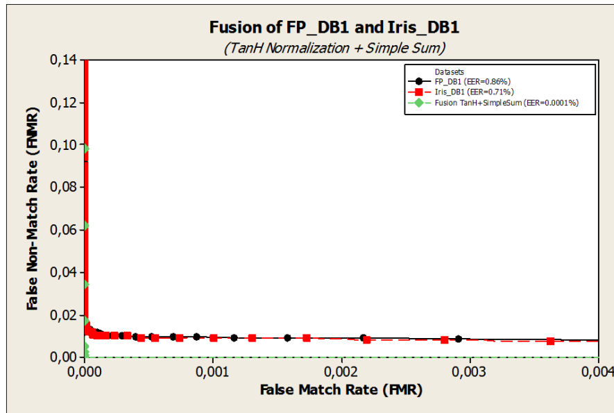
Figure 71: Scenario 1: Multi-modal Performance of Fingerprint and Iris using TanH Score Normalization + Simple Sum Score Fusion. EER_{FP\_DB1} = 0.86\% , EER_{Iris\_DB1} = 0.71\% , EER_{Finger+Iris} = 0.00010\% .
