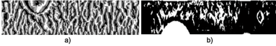
Figure 33: An example of a) iris code and b) iris mask. Calculated by Matlab (from CASIA DB image sample).
