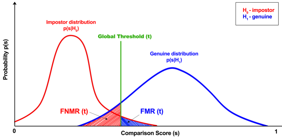
Figure 59: Biometric system comparison score distributions.
