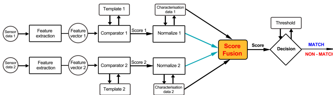
Figure 40: Advanced framework for score-level fusion approach [7].
