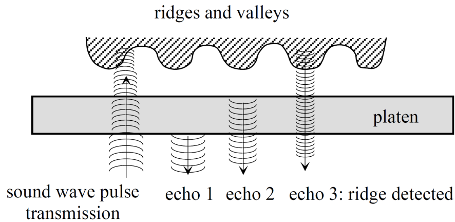
Figure 12: Ultrasound sensor (basic principle) [1].
