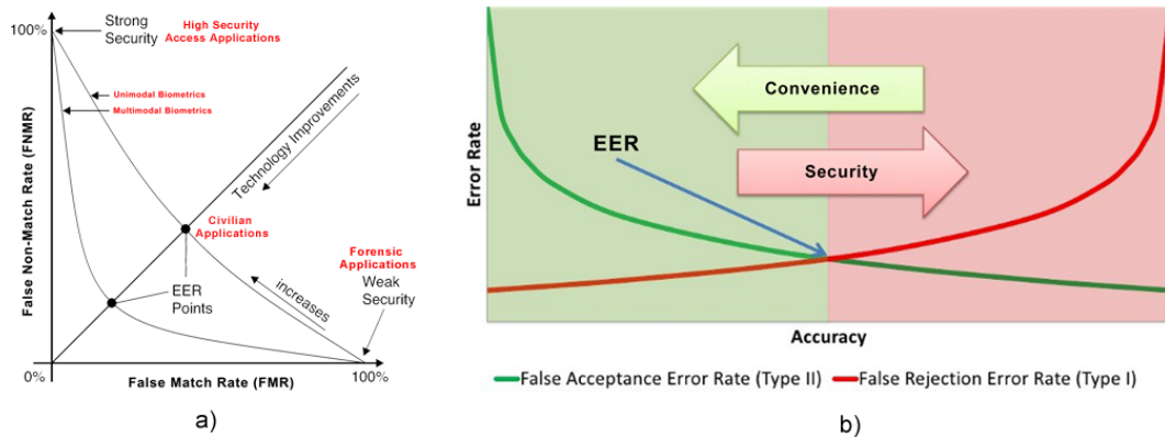
Figure 62: Security vs. Convenience a) Unimodal and multimodal biometrics in different applications. b) Illustration of Security vs. Convenience.
