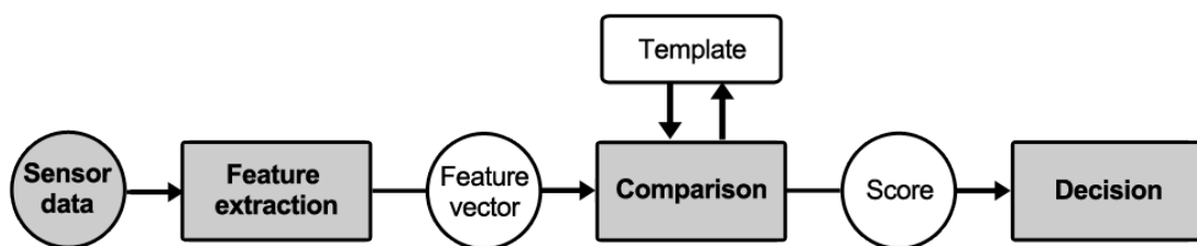
Figure 35: General biometric authentication process flow.
