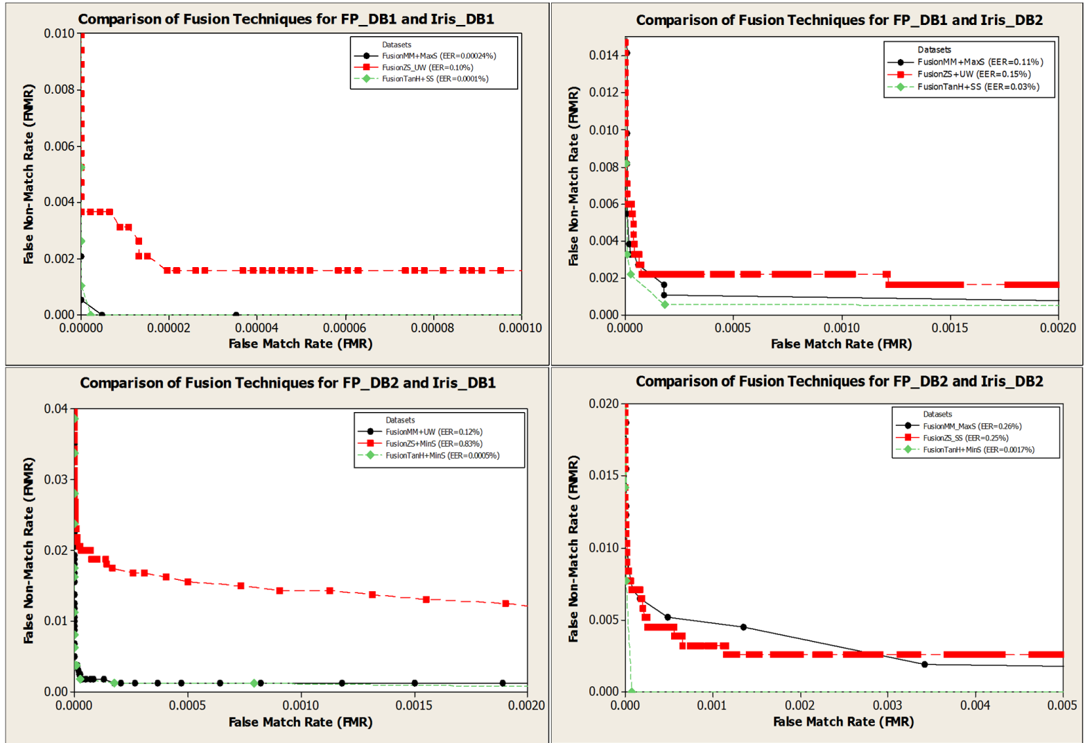
Figure 75: Comparison of Normalization and Fusion Techniques.
