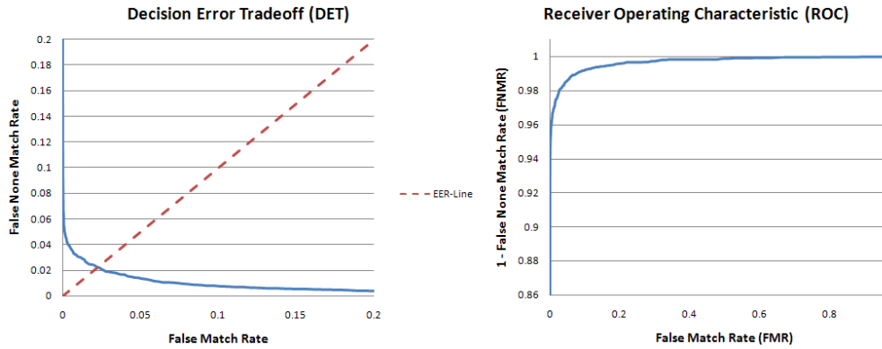
Figure 61: An example of Decision Error Trade-off (DET) and Receiver Operating Characteristic (ROC) curves [30].
