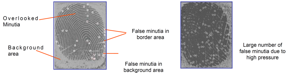
Figure 14: Poor image quality fingerprint image acquisition challenge [3].
