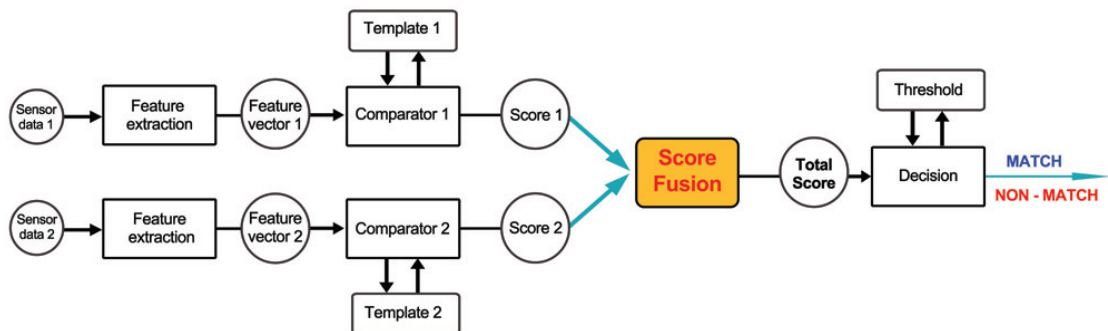
Figure 38: Fusion at comparison score level [7].
