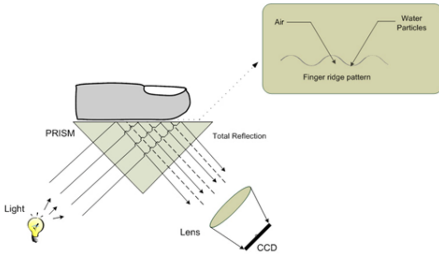
Figure 10: Optical fingerprint capture by FTIR (Frustrated Total Internal Reflection) [2].
