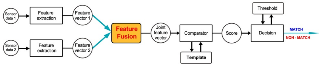
Figure 37: Fusion at feature-extraction level [7].
