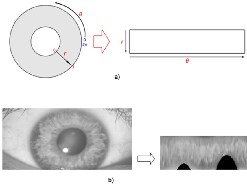
Figure 31: Iris Normalization. a) Daugman's Rubber Sheet Model, b) Example of iris image and normalized iris.
