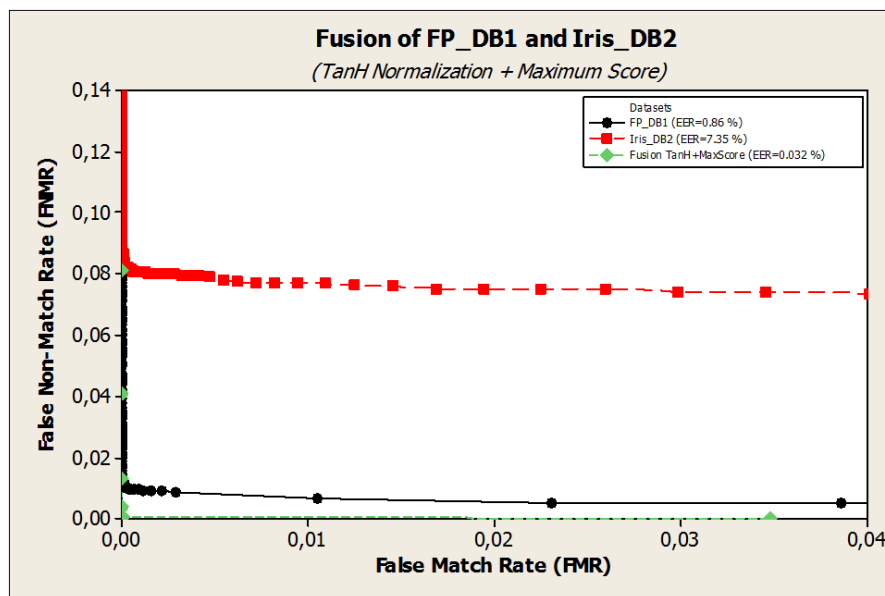
Figure 72: Scenario 2: Multi-modal Performance of Iris and Fingerprint using TanH Score Normalization + Maximum Score rule Fusion. EER_{FP\_DB1} = 0.86\% , EER_{Iris\_DB2} = 7.35\% , EER_{Finger+Iris} = 0.0320\% .
