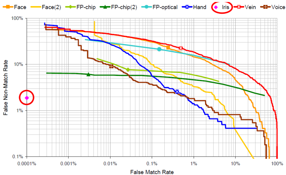
Figure 1: Detection Error Trade-off (DET): False Match rate (FMR) vs. False Non-Match Rate (FNMR) [22].
