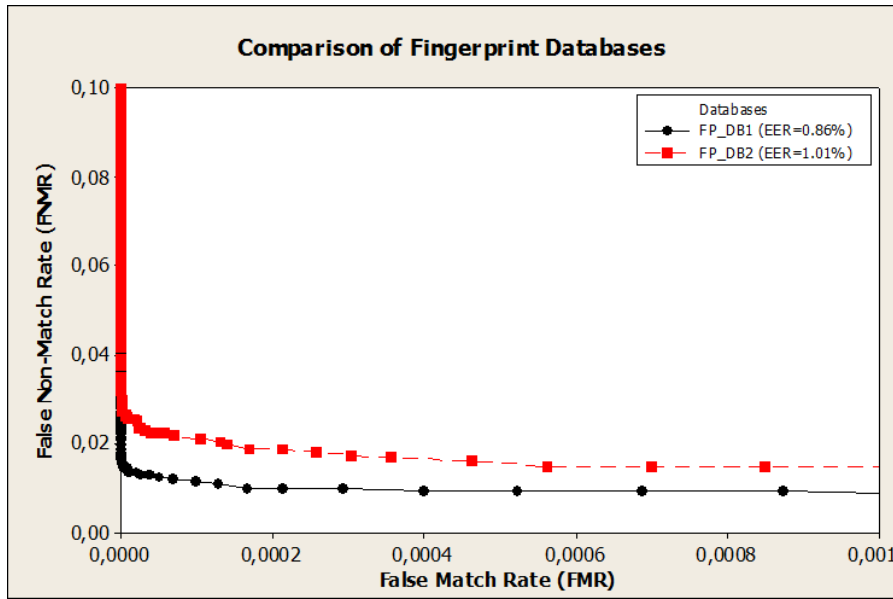
Figure 68: Comparison of Fingerprint Databases. EER_{FP\_DB1} = 0.86\% and EER_{FP\_DB2} = 1.01\% .
