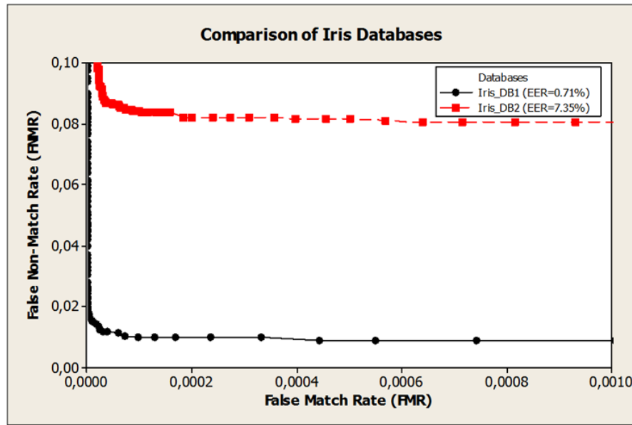
Figure 69: Comparison of Iris Databases. EER_{Iris\_DB1} = 0.71\% and EER_{Iris\_DB2} = 7.35\% .
