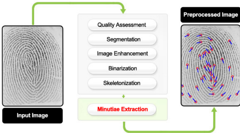
Figure 20: Flow diagram of the minutia-based pre-processing technique.
