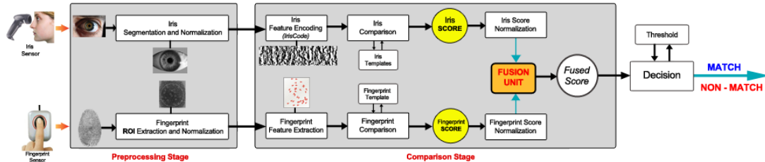
Figure 63: Our Approach: Score-Level Fusion of Fingerprint and Iris Recognition.
