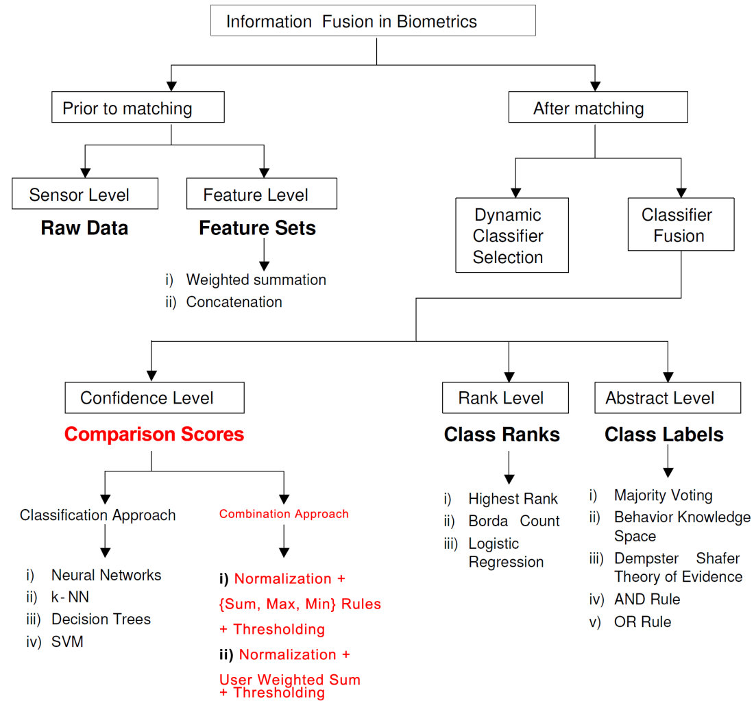
Figure 41: Summary of fusion levels and techniques in multi-modal biometrics.
