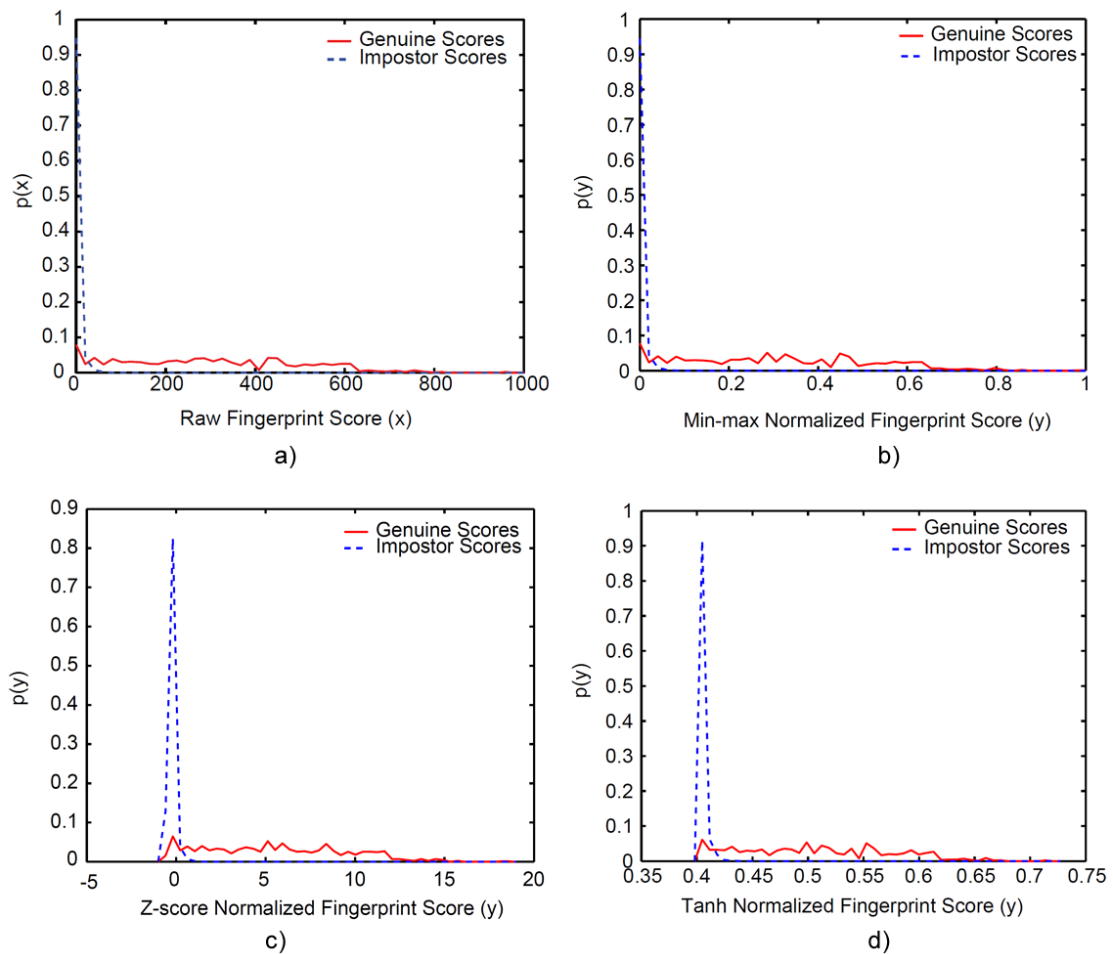
Figure 64: Distributions of genuine and impostor comparison scores. a) Fingerprint un-normalized scores b) MinMax normalization, c) Z-Score normalization and d) TanH normalization.
