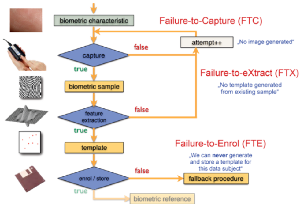
Figure 58: Potential failures in a biometric processing pipeline.
