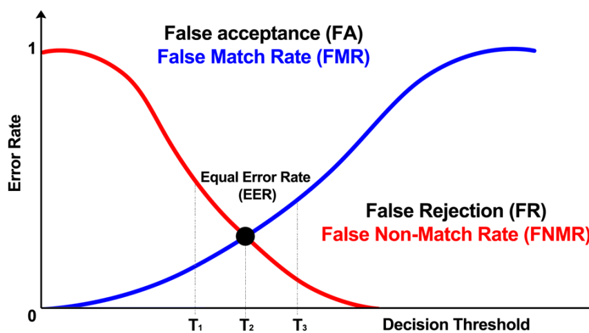
Figure 60: An example of EER point.
