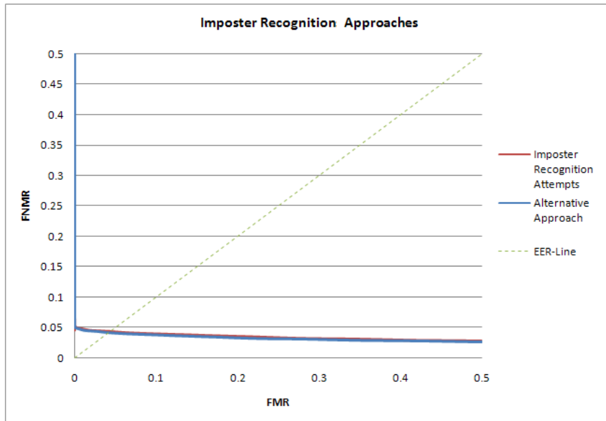
Figure 66: DET-curve illustrating impostor recognition and alternative impostor recognition.
