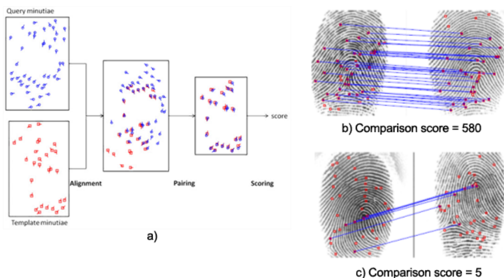
Figure 21: Fingerprint comparison by VeriFinger SDK 6.5. a) Flow diagram of a minutiae-based comparison algorithm. b) A genuine comparison of fingerprints with 30 matched minutiae, and c) an imposter comparison with 5 matched minutiae. Matched minutiae are connected by blue lines. The comparison score (is calculated based on matched minutiae and some other functions that are defined by Neurotechnology.
