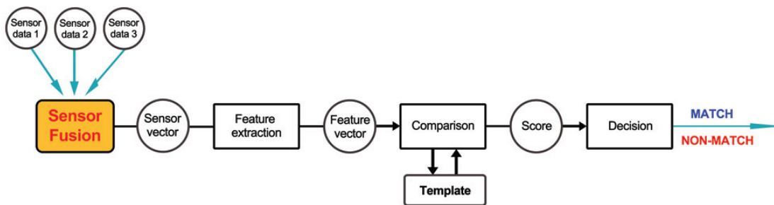
Figure 36: Fusion at sensor level [7].
