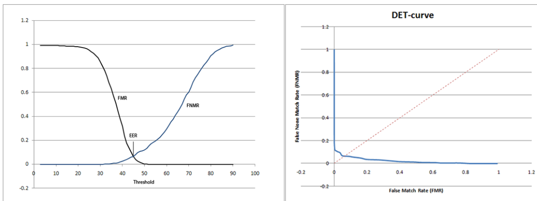
Figure 65: Calculating EER from FMR / FNMR intersection.
