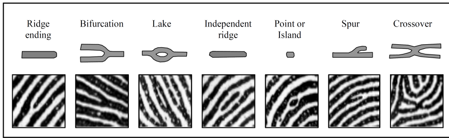
Figure 17: The most common fingerprint minutiae features (Galton classification) [1].
