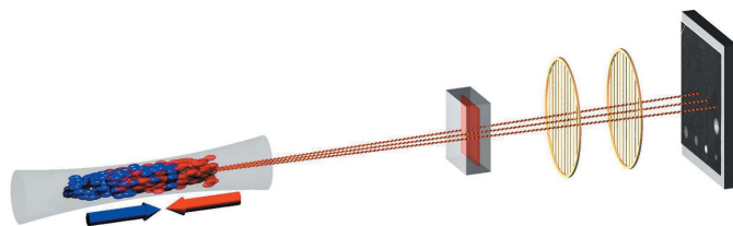
Figure 1 The Compact Light Source consists of an electron storage ring and a laser cavity. At the interaction point of the counter-propagating electron bunch (blue) and laser pulse (red), hard X-rays are produced in the process of inverse Compton scattering. The X-rays, which are emitted in a cone, shine onto the sample. The grating interferometer consists of two gratings and a PILATUS detector.
