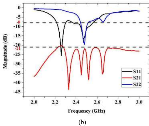
Fig. 11. (a) Fabricated prototype. (b) Measured S-parameter.
