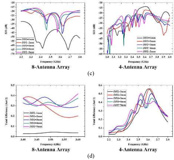
Fig. 12. The impact of a metal housing and a USB connector. (a) Simulation models. (b) Reflection coefficients, (c) mutual coupling, and (d) total efficiency of Ant 2 in the 8-antenna array and Ant 1 in the 4-antenna array.
