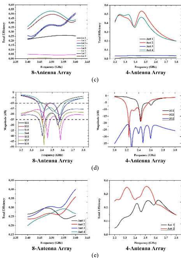
Fig. 13. The effect of a user's hand(s). (a) Two typical usage scenarios. (b) S-parameter and (c) total efficiency of the 8-antenna array and 4-antenna array at SHO mode. (d) S-parameter and (e) total efficiency of the 8-antenna array and 4-antenna array at DHO mode. All the results were obtained from HFSS.
