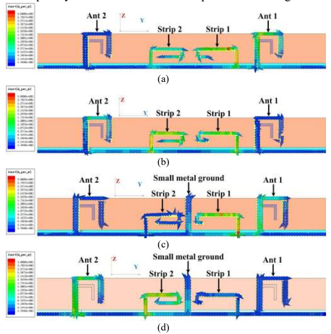
Fig. 5. Current distributions. (a) Strip 1 and (b) Strip 2 resonates without small metal ground. (c) Strip 1 and (d) Strip 2 resonates with small metal ground.
