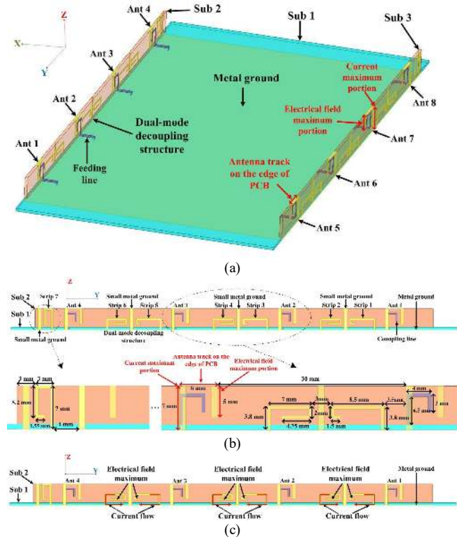
Fig. 6. Configuration of the 8-antenna array. (a) Overall view. (b) Detailed dimensions. (c) The arrangement of the energy maximum portions.
