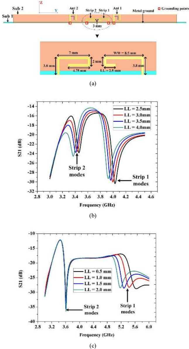
Fig. 2. An example for mutual effect. (a) Configuration. (b) S_{21} when WW = 8.5 mm. (c) S_{21} when WW = 5 mm.
