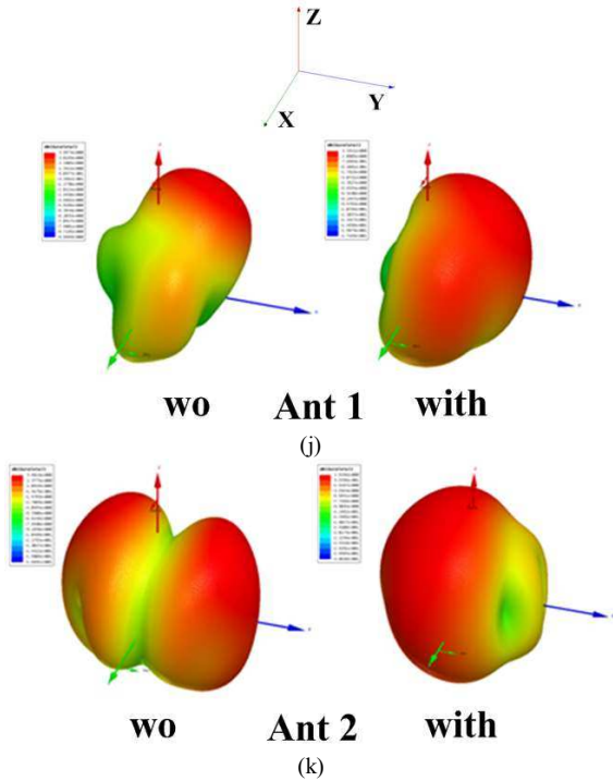
Fig. 10. Simulated results. (a) S11/S22 and (b) S12 with/without decoupling elements obtained from HFSS. (c) RE and (d) TE with/without decoupling elements from HFSS. (e) RE and TE with decoupling elements from CST. Resonant frequency of (f) Strip 1, (g) Strip 2, (h) Strip 3, and (i) Strip 4 changes obtained from HFSS. 3D antenna patterns of (j) Ant 1 at 2.5 GHz and (k) Ant 2 at 2.4 GHz with and without decoupling elements obtained from HFSS.
