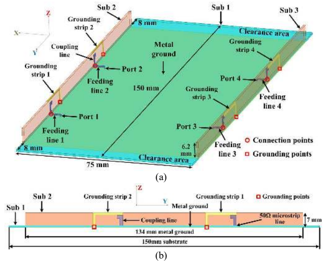
Fig. 1. Configuration of an antenna array. (a) Overall view. (b) Side view.
