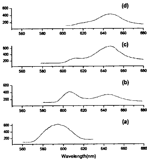
Fig. 2. Shift of fluorescence emission peak due to energy transfer process in dye mixture doped POF: (a) Rh 6G (0.25 mM), (b) dye mixture Rh 6G (0.25 mM) and Rh B (0.11 mM), (c) dye mixture Rh 6G (0.25 mM) and Rh B (0.25 mM), and (d) Rh B (0.25 mM). Pump energy is 0.12 mJ/pulse. Length of the POF is 7 cm and diameter 510 \mu\text{m} .
