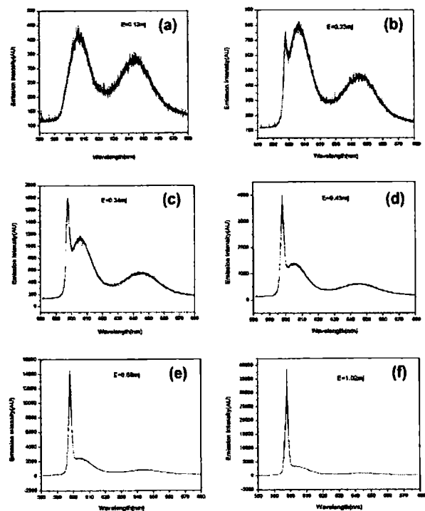
Fig. 3. Emission from 510 \mu\text{m} diameter and 7 cm long dye doped POF at a pump energy of (a) 0.12, (b) 0.23, (c) 0.34, (d) 0.43, (e) 0.68, and (f) 1.02 mJ.
