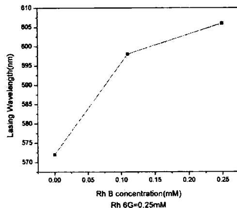
Fig. 4. Tuning of multimode laser emission peak with different dye concentrations. Rh 6G concentration is constant (0.25 mM) in all three samples. Pump energy is 1.37 mJ/pulse. L = 7 cm and D = 510 \mu\text{m} .
