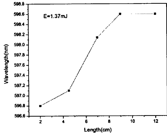
Fig. 8. Variation of laser emission peak with length of the fiber having a diameter of 510 \mu\text{m} at a pump energy of 1.37 mJ/pulse.
