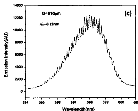
Fig. 6. Multimode laser emission from 7 cm long dye doped fiber at a pump energy 1.37 mJ/pulse. D = (a) 335, (b) 405, and (c) 510 \mu\text{m} .
