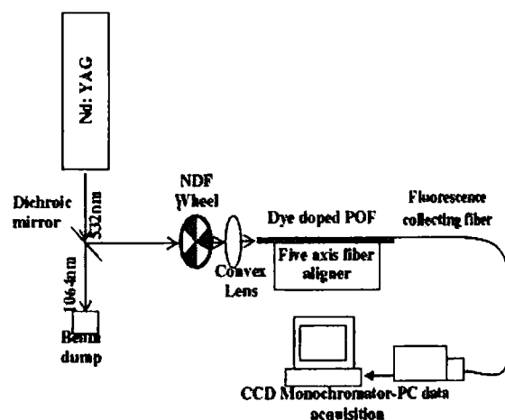
Fig. 1. Experimental setup to record the fluorescence emission from the fiber end. Pumping is done axially.
