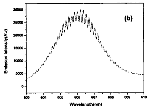
Fig. 5. (a) Typical multimode laser emission spectrum at a pump energy of 0.47 mJ/pulse from a POF doped with equal concentrations (0.25 mM) of Rh 6G and Rh B. (b) Expanded modes in (a).
