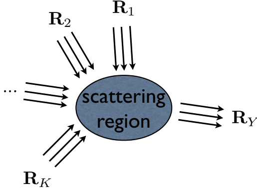
FIG. 1. (Color online) Graphical representation of the scheme underlying the multimode QEPI (10): it establishes a lower bound on the von Neumann entropy emerging from the output port indicated by \mathbf{R}_Y of a multimode scattering process that linearly couples K independent sets of bosonic input modes (each containing n modes), initialized into factorized density matrices.
