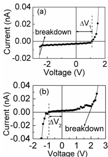
Figure 4 | Zoomed-in I - V characteristics of (a) for processes (1) and (2), and (b) for processes (3) and (4) under a current compliance of 10 nA. I - V characteristic in (a) shows the ordinary behavior for a forward-biased diode, while in (b) it is the one for a reversed-biased diode. The turn-on voltages are V_1 (1.1 V) and V_2 (0.9 V) for the forward-biased and reversed-biased diodes, respectively. Breakdown characteristics of the diodes are also evident.
