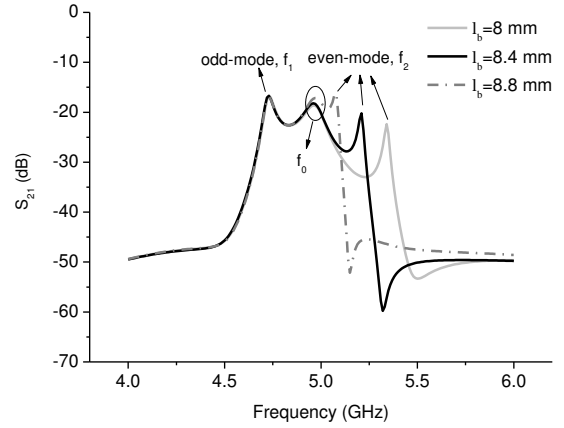
Fig. 6 The change of the resonant frequencies of the structure in Fig. 3 with l_b .
