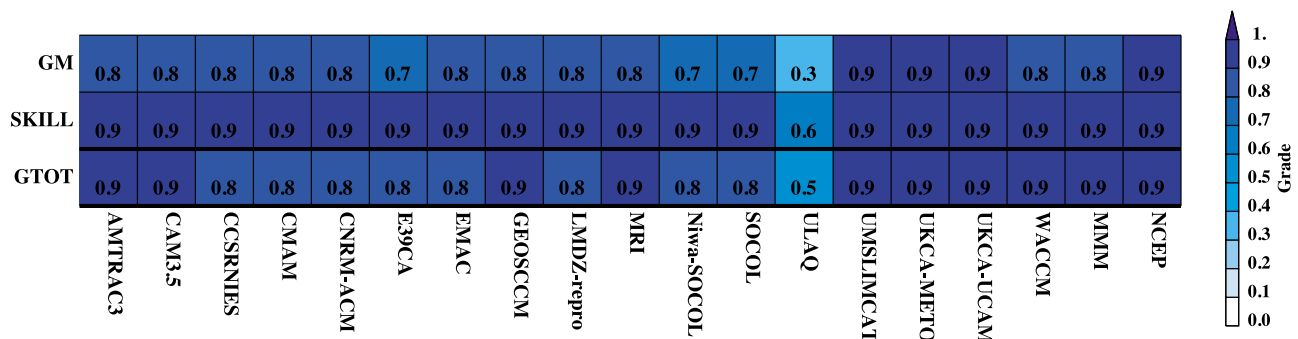
Figure 5. Same as Figure 4 but for JJA.
