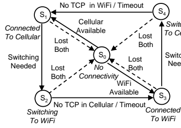
Figure 7. State Diagram.
