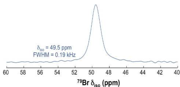
Figure 1. ^{79}\text{Br} MAS NMR spectrum obtained at 14T on \text{MAPbBr}_3 .
