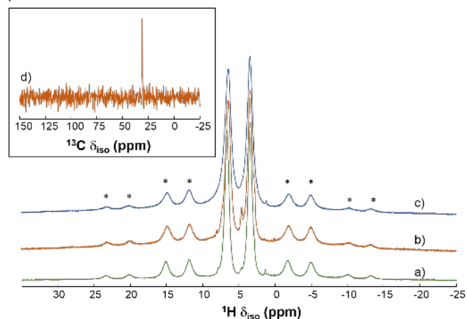
Figure 4. 1 H MAS NMR spectra obtained at 14 T under MAS condition for MAPbCl 3 (a), MAPbBr 3 (b) and MAPbI 3 (c). Spinning sidebands are marked with asterisks. Insert: 13 C CPMAS spectra obtained on MAPbBr 3 .
