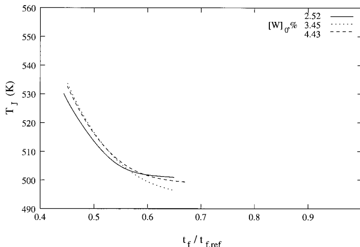
Figure 8 Jacket fluid temperatures corresponding to different points on the three Paretos.
