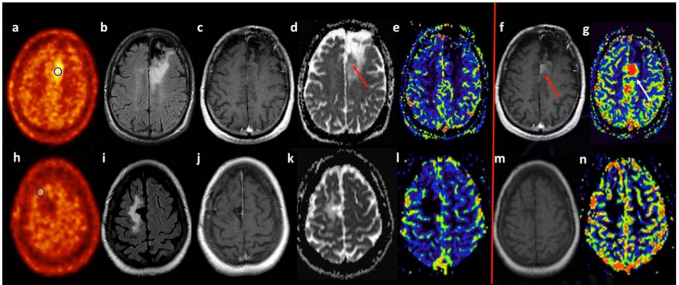
Figure 4. Correlation between tumour-to-normal brain (T/N) ratio 6- ^{18}\text{F} -fluoro-L-3,4-dihydroxyphenylalanine ( ^{18}\text{F} -FDOPA) positron emission tomography (PET) uptake and outcome: the top row is showing a case of a left frontal low-grade glioma (LGG) with ^{18}\text{F} -FDOPA PET images (a) during follow-up, demonstrating a high T/N ratio of 2.5 in the hotspot region (circle). A close MR examination is demonstrating a fluid-attenuated inversion-recovery (FLAIR) hyperintense lesion (b), without contrast enhancement (c) and with a small area of hypointensity on apparent diffusion coefficient (ADC) maps (d) (arrow), without increase in the relative cerebral blood volume (rCBV) values on CBV maps (e). Follow-up MR scan 1 year later is demonstrating the presence of a focus of enhancement (f) (arrow) and high rCBV values within the lesion (g) (arrow) consistent with disease progression. The bottom row is showing a companion case of a right frontal LGG with low values of T/N ratio (1.2) at ^{18}\text{F} -FDOPA PET images (h) (circle). Close MR scan demonstrated an area of FLAIR hyperintensity (i) without contrast enhancement (j) or evidence of decreased ADC (k) or increased rCBV values (l). Follow-up MR scan 1 year later is demonstrating unmodified radiologic findings on post-contrast T_1 weighted images (m) and rCBV maps (n), suggesting stable disease.
