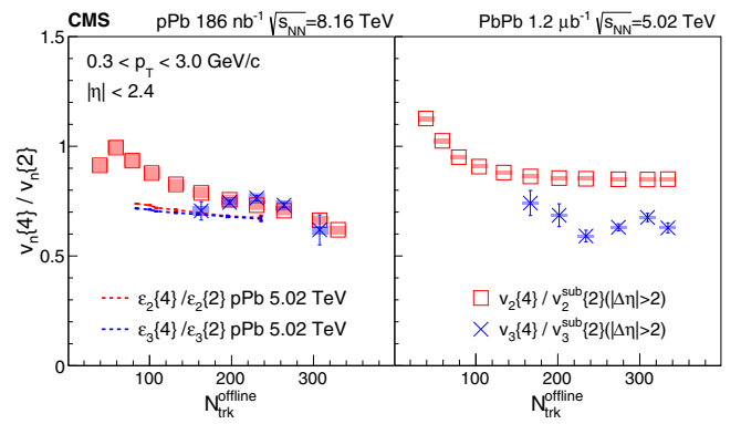
FIG. 2. The ratios of four- and two-particle harmonics ( v_2\{4\}/v_2\{2\} and v_3\{4\}/v_3\{2\} ) shown for p\text{Pb} \sqrt{s_{NN}} = 8.16 TeV (left) and \text{PbPb} \sqrt{s_{NN}} = 5.02 TeV (right) collisions as a function of N_{\text{trk}}^{\text{offline}} . Error bars and shaded boxes denote statistical and systematic uncertainties, respectively. The dashed curves show a hydrodynamics-motivated initial-state fluctuation calculation of eccentricities \varepsilon_n\{m\} for p\text{Pb} collisions at \sqrt{s_{NN}} = 5.02 TeV [45].
