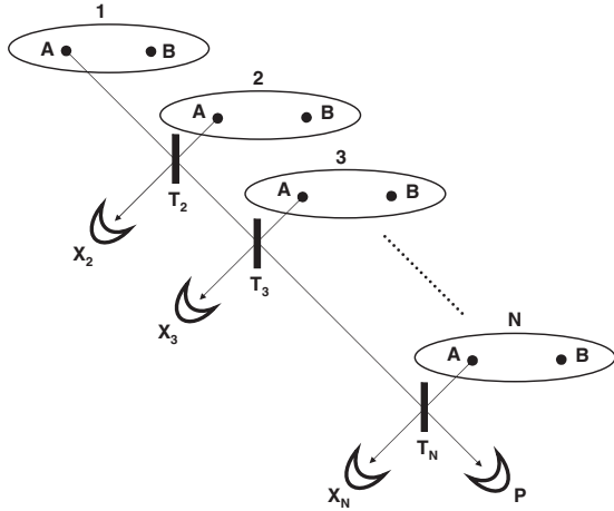
FIG. 1. Multipartite entanglement swapping. We start from N independent copies of the state \rho_{AB} . The A systems are sent to a relay for a multipartite CV Bell detection. The latter is an interferometer with a suitable cascade of beam splitters, followed by homodyne detections ( N - 1 in the X quadratures, and a final one in the P quadrature). The outcomes \gamma are broadcasted to the users, so that their multipartite state collapses into a conditional cluster state \rho_{B_1 \dots B_N | \gamma} . The transmissivities T_k of the beam splitters are chosen so that the cluster state is invariant under permutation of the users.
