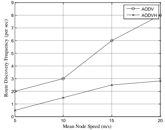
Figure 14. Route Discovery with Mobility
