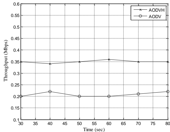
Figure 17. Throughput vs. Time (FSO Only Path)
