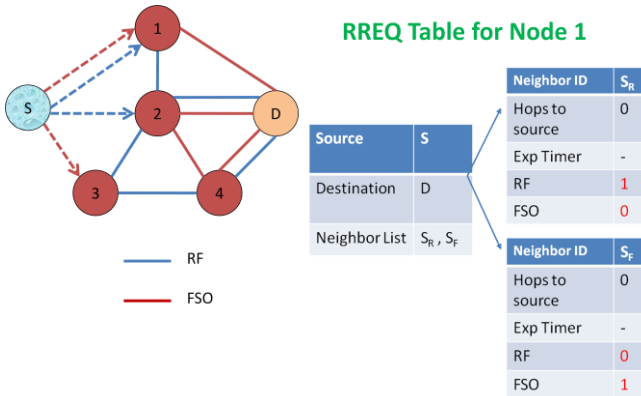
Figure 6. RREQ Table for Node 1 (stage 1)
