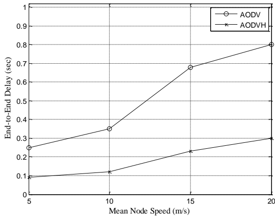
Figure 13. End-to-End Delay with Mobility
