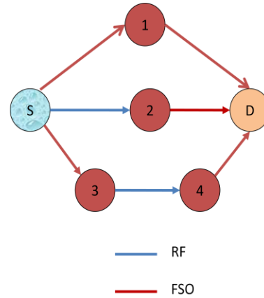
Figure 11. Forward Path Setup from Source S
