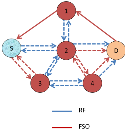
Figure 9. RREP Reaching Source Node S
