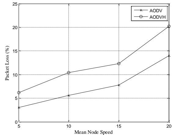
Figure 12. Packet Loss with Varying Mobility
