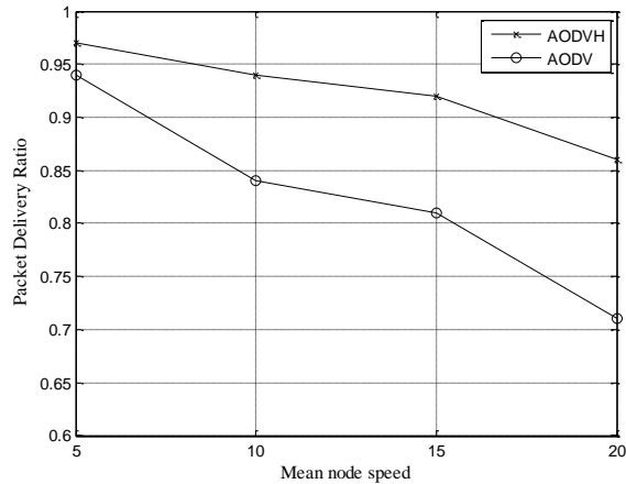
Figure 15. Packet Delivery with Mobility
