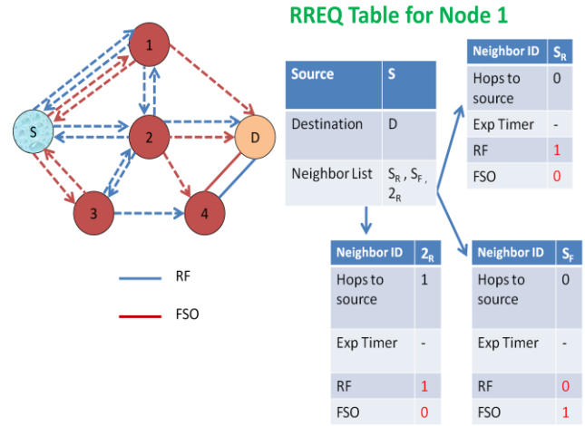
Figure 7. RREQ Table for Node 1 (Stage 2)
