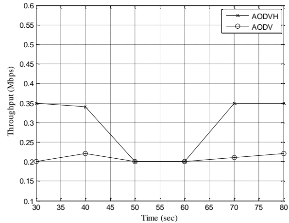
Figure 18. Throughput vs. Time (Hybrid Path)
