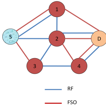
Figure 5. Topology for AODV
