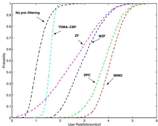
Fig. 3. CDF of rates, SNR = 10\text{dB} , per user, M = 3 , N = 3 , Rayleigh 3 \times 3 channel.
