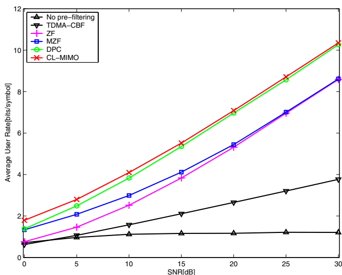
Fig. 2. Average rate per user vs. SNR, M = 3 , N = 3 , Rayleigh 3 \times 3 channel.
