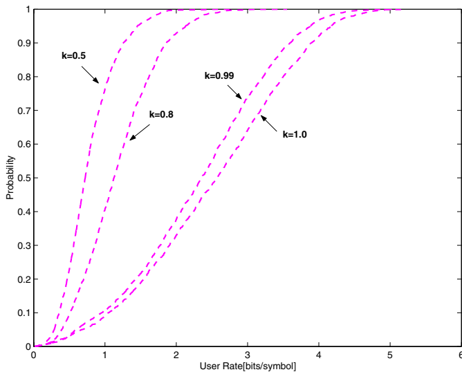
Fig. 5. CDF of rates for different correlation k = 0.5, 0.8, 0.99, 1 , SNR = 10\text{dB} , M = 3 , N = 3 , Rayleigh 3 \times 3 channel.
