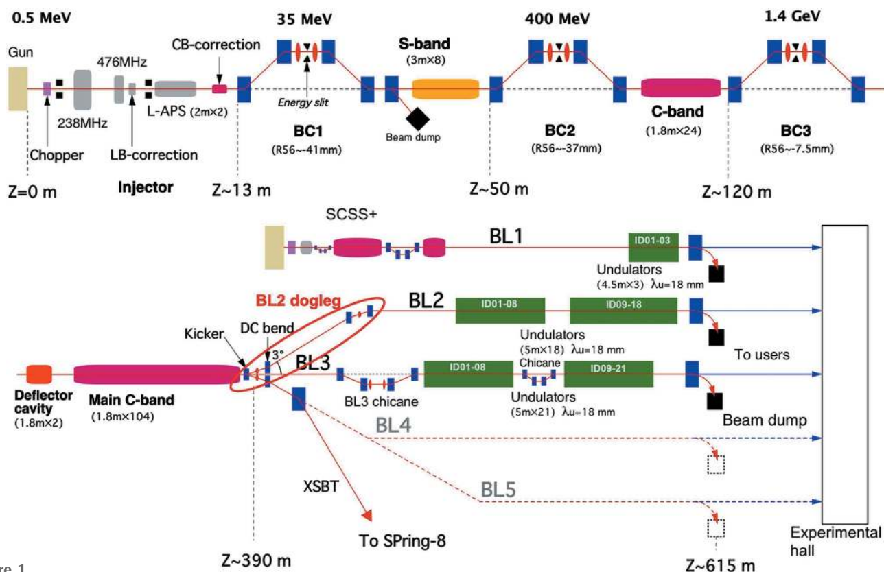
Figure 1 Schematic layout of the SACLA accelerator.
