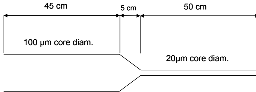
Figure 58: Tapered fiber geometry for SBS threshold reduction
