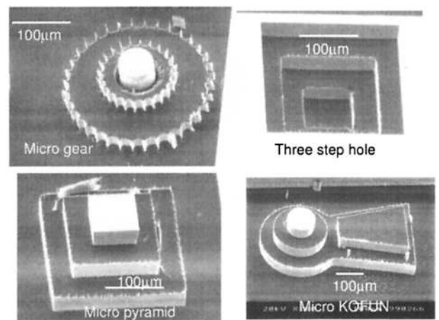
Fig. 4. SEM view of three level structure
