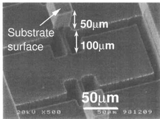
(b) Delay-masking process for multi-height structure
