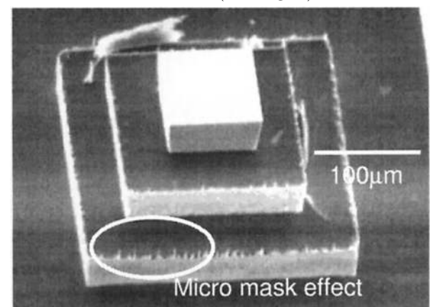
Fig. 8. SEM view of micro mask
