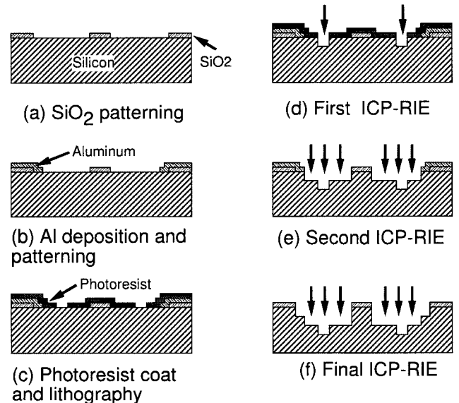
Fig. 3. Process Flow of triple DMP
