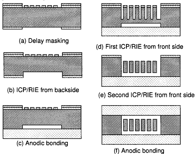
Fig. 5. DMP with bonding process
