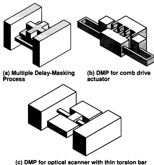
Fig.9. Example of 3-D structure by multiple DMP
