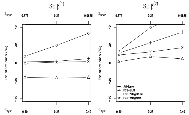
FIG. 1. Robustness to the proportion of systematically missing values: estimate of the relative bias for the SE estimate for \beta^{(1)} (left), \beta^{(2)} (right) according to \pi_{\text{syst}} for each MI method. The estimated relative bias is calculated by the difference between the model SE and the empirical SE, divided by the empirical SE. The proportion of sporadically missing values is accordingly modified to keep a constant proportion of missing values (in expectation).
