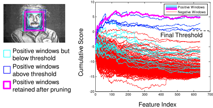
Figure 1: Traces of cumulative scores of different windows in an image of a face. See text.
