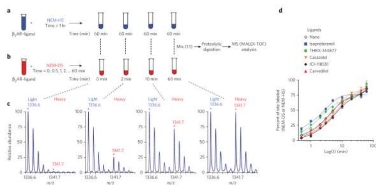
Figure 3. Schematic illustration of time-dependent, residue-specific labeling experiment designed to monitor conformational changes in the \beta_2 AR
