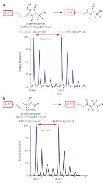
Figure 1. Labeling of cysteines and lysines in the \beta_2\text{AR} to monitor conformational changes (a) top, reaction of thiolate anion of cysteine side chain with N -ethylmaleimide (neM-H 5 or neM-d 5 ) by nucleophilic addition at the double bond of the maleimide ring. bottom, representative isotope-peak pair (doublet) corresponding to a chymotryptic peptide ( ^{125}\text{cviAvdRYF}^{133} ) modified at cys125 by a light and heavy neM ( m/z 1210.6 and 1215.6, respectively; \sim\Delta m/z = 5 ). (b) top, reaction of the \epsilon -nH 2 group of the lysine side chain with succinic anhydride (SA-H 4 or SA-d 4 ) by nucleophilic addition at one of the carbonyl groups. bottom, representative spectrum of doublet peaks corresponding to a chymotryptic peptide ( ^{259}\text{RRSSKF}^{264} ) modified at lys263 by light and heavy succinic anhydride ( m/z 880.5 and 884.5, respectively; \sim\Delta m/z = 4 ).
