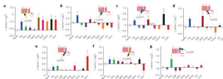
Figure 5. Reactivities of residues in \beta_2 AR featuring ligand-specific conformational rearrangements
