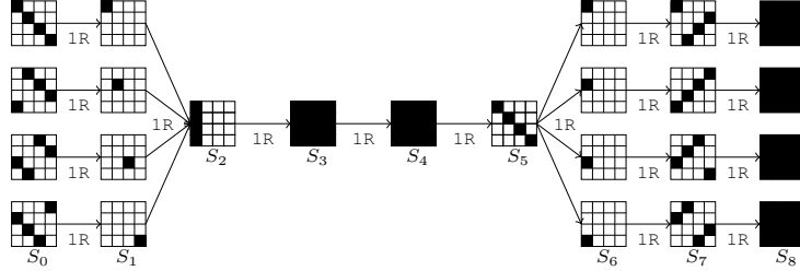
Figure 5: Differential characteristic for the 8-round known-key distinguisher for AES-128
