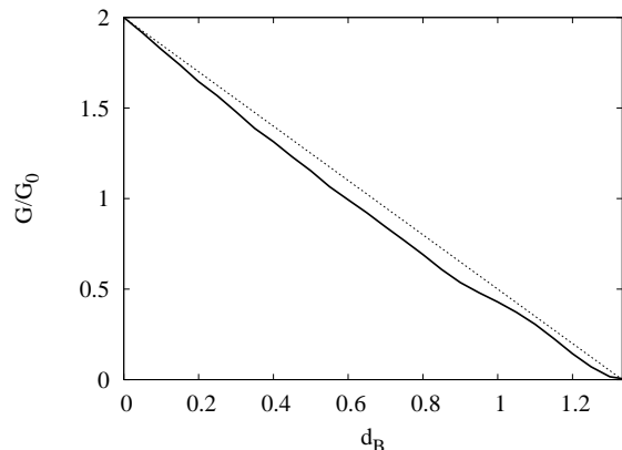
FIG. 8: The conductance as a function of d_B for N = 3 barriers with E = 2 and d_0 = 10 (solid line). The dashed line is the curve given by the classical limit Eq. (16).
