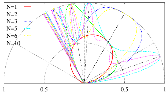
FIG. 10: (Color online) Angular dependence of the transmission probability at E = 1 and d_B = d_{-B} = 1 for several values of N . The black dashed lines correspond to the angles for recursive transmission of multiplicity 2 (at \phi \approx \pi/18 ), 3 (at \phi = -\pi/6 ) and 5 (at \phi \approx -\pi/54 and \phi \approx -7\pi/18 ).
