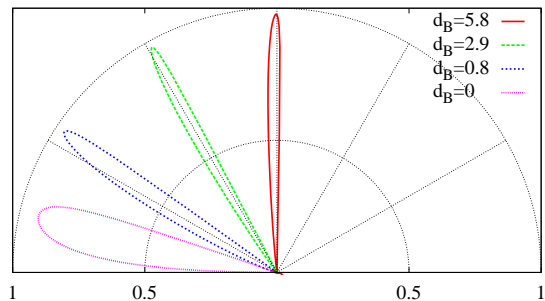
FIG. 9: (Color online) Angular dependence of the transmission probability at E = 6 through a structure consisting of one magnetic barrier of width d_B and one magnetic well of width d_{-B} . We fix d_{-B} = 11.7 \approx 2E and vary d_B from 0 to 5.8 \approx E .
