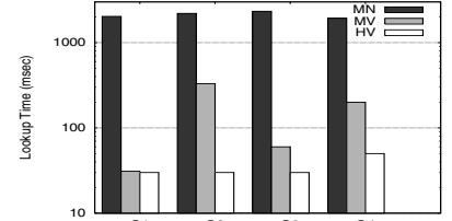
Fig. 9. Lookup Time
