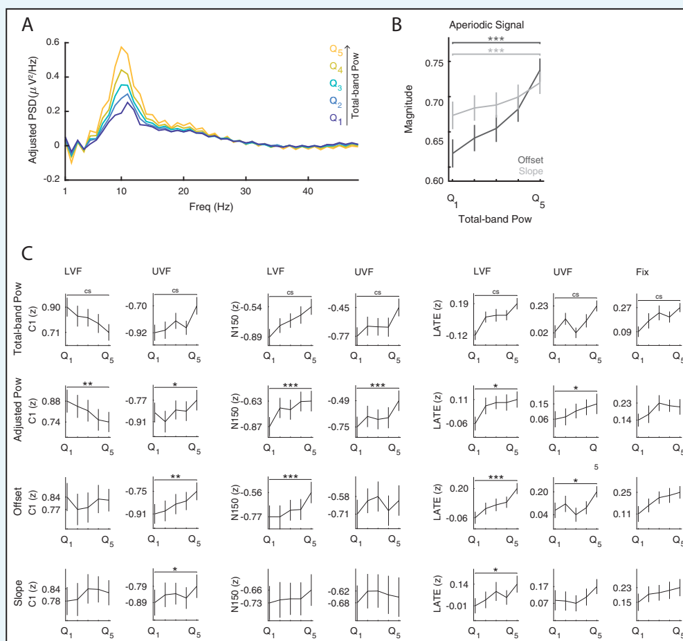
Appendix 1—figure 1. Analysis of periodic and aperiodic features of the prestimulus power spectrum. (A) Group-average prestimulus aperiodic-adjusted power spectrum shown separately for the five bins sorted from weak ( Q_1 ) to strong ( Q_5 ) total-band power. (B) Group-average offset (dark) and slope (light) of the aperiodic signal sorted from weak ( Q_1 ) to strong ( Q_5 ) total-band power. The results in A and B are shown for the frequencies and electrodes of most positive/negative t-statistics, collapsed across the significant clusters of Figure 3 . (C) Group-average normalized ERP amplitude on trials sorted by total-band power, aperiodic-adjusted power, offset and slope. ERP amplitudes were compared across most extreme bins ( Q_{5-1} ) at the ERP time point and the prestimulus-power electrode and frequency of most positive/negative t-statistics, separately for each component and trial type. ***, **, * indicate FDR-corrected p-values < 0.001, 0.01, 0.05, respectively. cs indicates significant p-values based on cluster-level statistics (see Figure 3 ).
