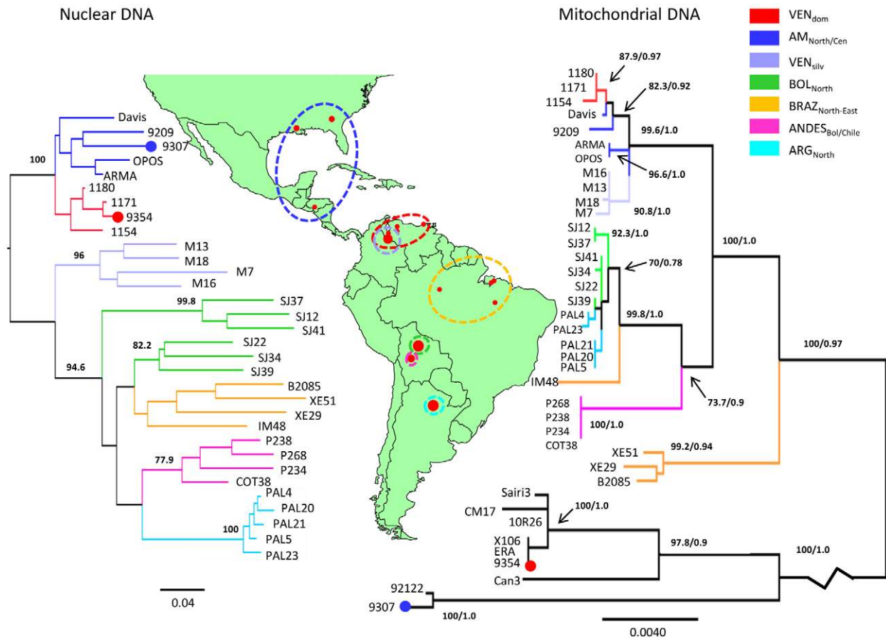
Figure 3. Unrooted Neighbour-Joining tree based on D_{AS} values from nuclear loci (left) and Maximum-Likelihood tree from concatenated maxicircle sequences (right) showing TcI population structure across the Americas. A panel of 32 TcI isolates from seven nuclear populations was assembled for analysis. Origin of individual strains is shown on the map by small red circles. Large red circles correspond to multiple samples, isolated from the same geographical area. Branch colours indicate strain population. The nuclear tree was constructed from concatenated polymorphisms present within the SL-IR , GPI and 25 microsatellite loci. D_{AS} values were calculated as the mean across 1000 random diploid re-samplings of the dataset and those greater than 70% are shown on major clades. A Maximum-Likelihood topology was assembled from concatenated maxicircle sequences. Branches show equivalent bootstraps and posterior probabilities from consensus Maximum-Likelihood (1000 replicates) and Bayesian topologies, respectively. The maxicircle topology is rooted against additional outgroup strains from TcIII and TcIV. The blue and red circles on branches represent inter-lineage introgression events. The blue circle indicates that the maxicircle in a sylvatic TcI isolate from AM_{North/Cen} is most closely related to the maxicircle found in TcIV samples from the same area. The red circle shows that the maxicircle haplotype in a human VEN_{dom} strain is the same as those in TcIII and TcIV isolates from neighbouring areas of Venezuela, Bolivia and Colombia. Divergent maxicircle haplotypes at the intra-DTU level are also observed in BRAZ_{North-East} (IM48) and AM_{North/Cen} (ARMA and OPOS). Another incidence of nuclear-mitochondrial incongruence is demonstrated by the paraphyletic grouping of ARG_{North} among a subset of BOL_{North} isolates in the maxicircle tree, compared to its monophyletic placement in the nuclear phylogeny. doi:10.1371/journal.pntd.0001584.g003
