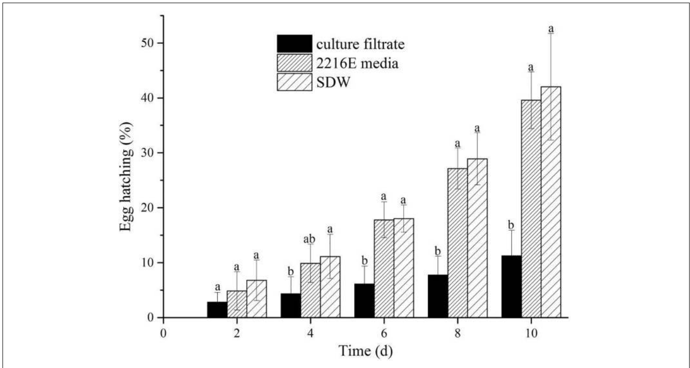
FIGURE 4 | Fumigation effects of original culture filtrates on egg hatching of M. incognita after 2, 4, 6, 8, and 10 days of incubation. Values with the same lowercase letters do not differ from each other at P < 0.05 ; bars indicate the standard error of the means ( n = 4 ).
