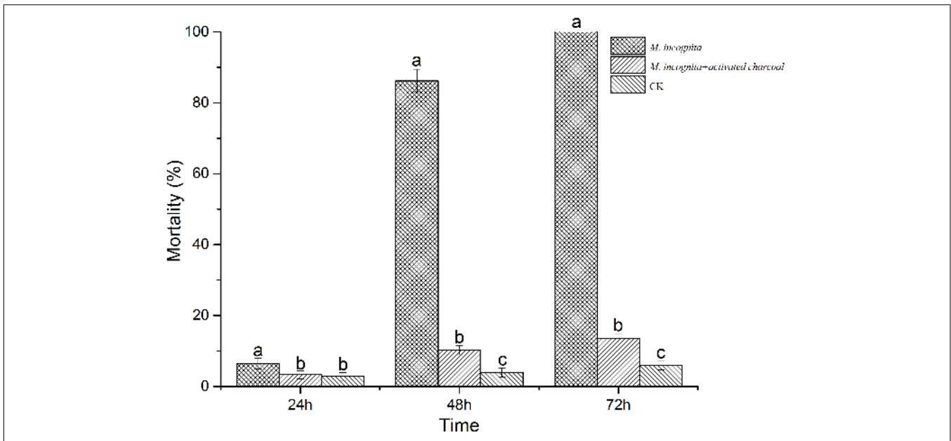
FIGURE 3 | Nematicidal effects of strain 1A00316 VOCs against M. incognita in a three-compartment Petri plate. Values with the same lowercase letters do not differ from each other at P < 0.05 ; bars indicate the standard error of the means ( n = 3 ).
