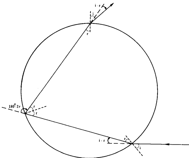
Fig. 3. Angles indicated are those needed to calculate the angle of deviation between the initial and final directions of a ray suffering one internal reflection.
