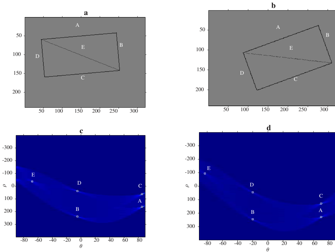
Figure 24: Effect of the transformation of maps on the Hough images a ) An example occupancy grid map. b ) The map is rotated 15^\circ and translated 50 cells along both axes. c ) Hough image of the map over 180 degrees. Labeled points correspond to the line segments. d ) Hough image of the transformed map over 180 degrees (Saeedi et al., 2014b).
