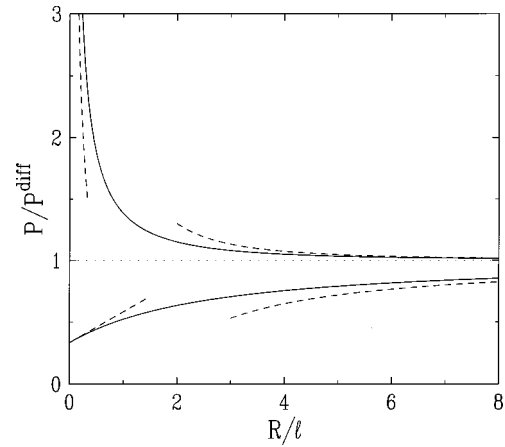
FIG. 13. Plot of the size factor P/P_{\text{diff}} of the polarizability of a transparent sphere (lower curves) and a reflecting sphere (upper curves): Solid lines, outcome of the numerical analysis; dashed lines, small-radius and large-radius behaviors of Table III.
