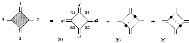
FIG. 14. Hikami four-point vertex. It describes the exchange of amplitudes of two incoming diffusions 1 and 3 into two outgoing diffusions 2 and 4. The dots linked with the dashed line denote an extra scatterer on which both amplitudes scatter. The solid lines are dressed amplitude propagators.
