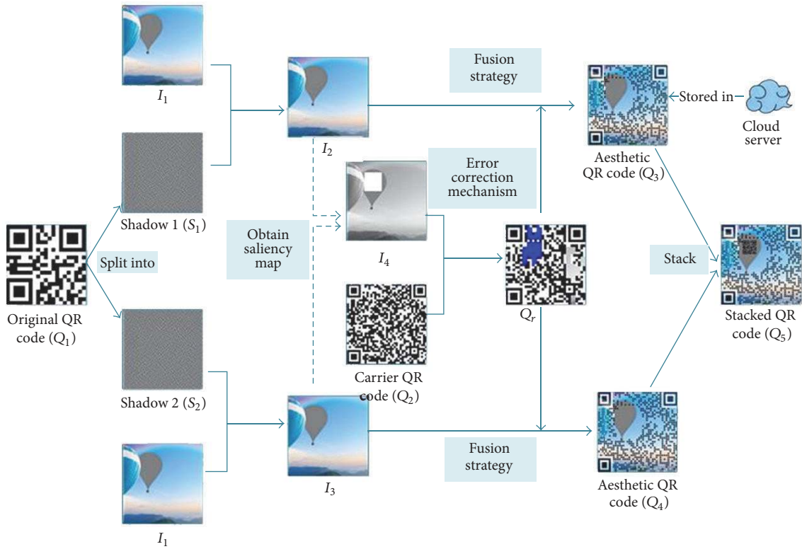
FIGURE 10: Flowchart of Scheme III.
