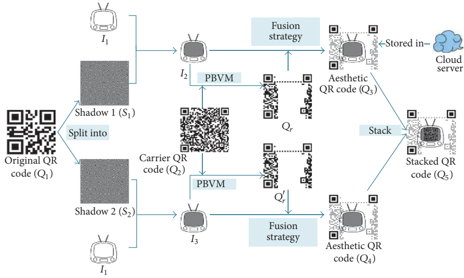
FIGURE 8: Flowchart of Scheme II.
