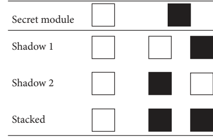
FIGURE 3: Construction of (2, 2) VCS scheme.
