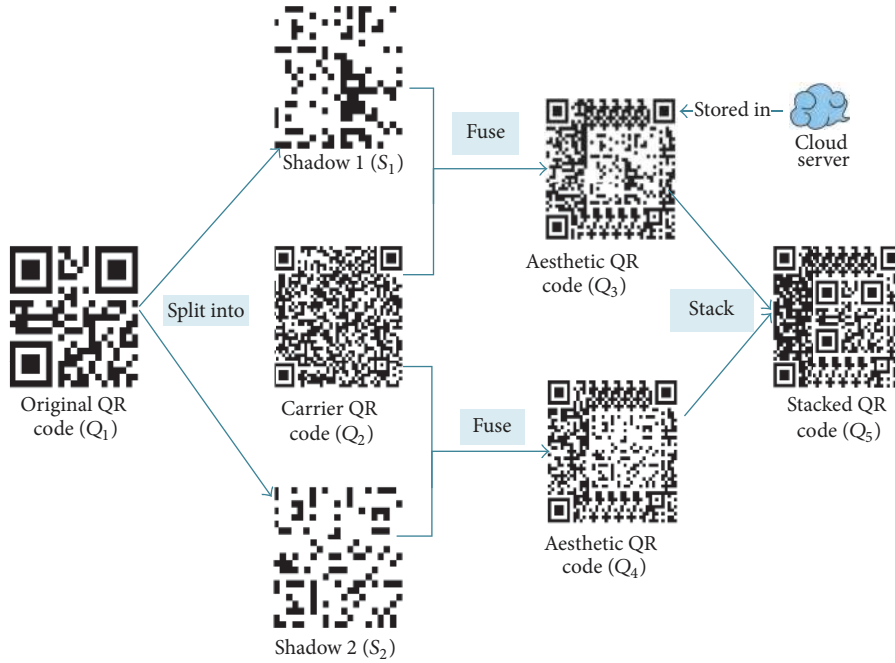
FIGURE 7: Flowchart of Scheme I.
