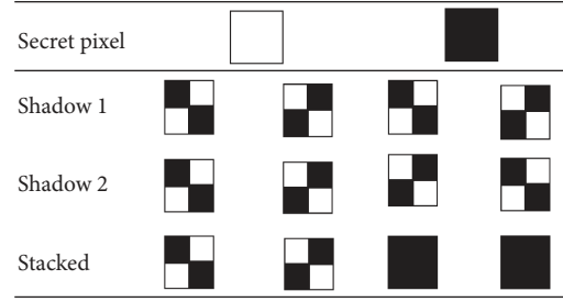
FIGURE 6: Nonexpansible VCS scheme.
