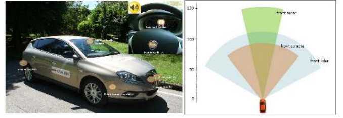
Figure 3. Left: images of the CRF vehicle demonstrator. Right: Field of view of the three frontal sensors used as inputs to gather datasets for our proposed fusion approach detailed in Sections VI, VII and VIII.
