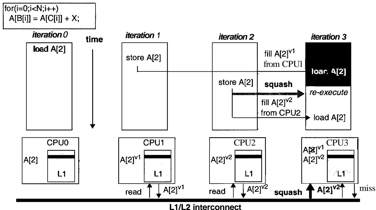
FIGURE 2: An example of implicit threading execution.
