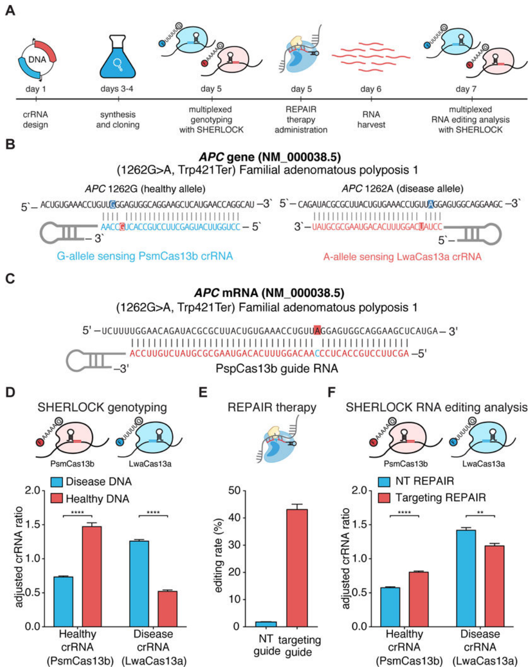
Figure 4. Combined therapeutics and diagnostics with Cas13 enzymes
