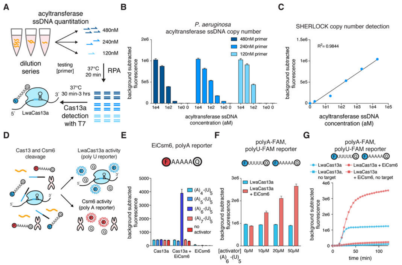
Figure 2. Single molecule quantitation and enhanced signal with SHERLOCK and Csm6
