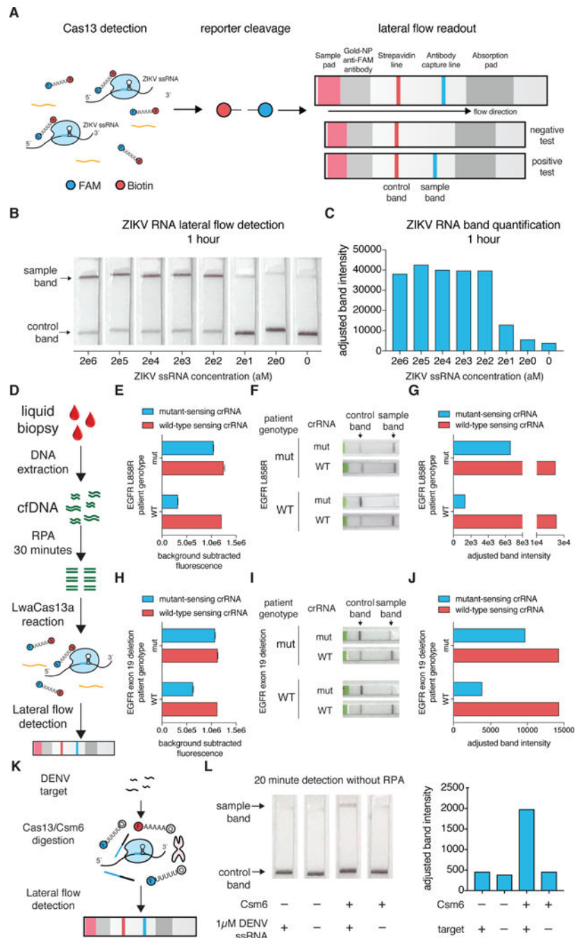
Figure 3. Adapting SHERLOCK for lateral flow detection
