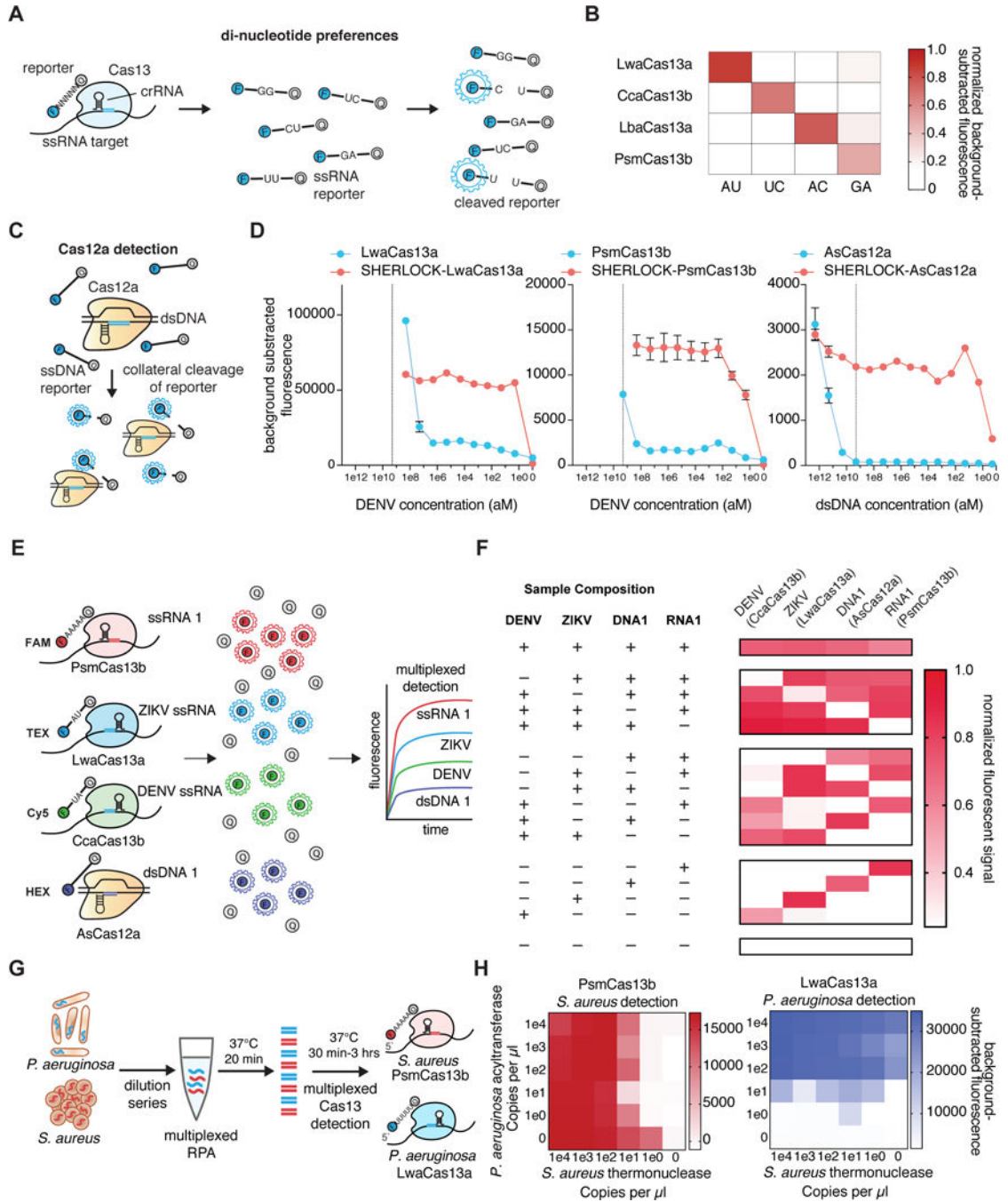
Figure 1. Multiplexed SHERLOCK detection with orthogonal collateral activity of Class 2 enzymes
