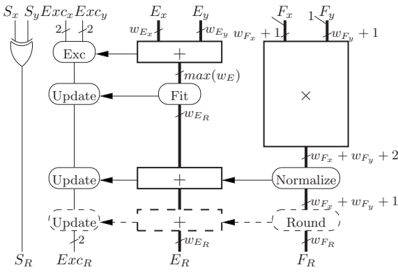
Figure 1: Architecture of a flexible floating-point multiplier
