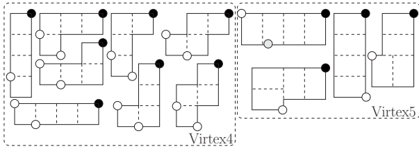
Figure 3: Some super-tiles exactly matching DSP blocks
